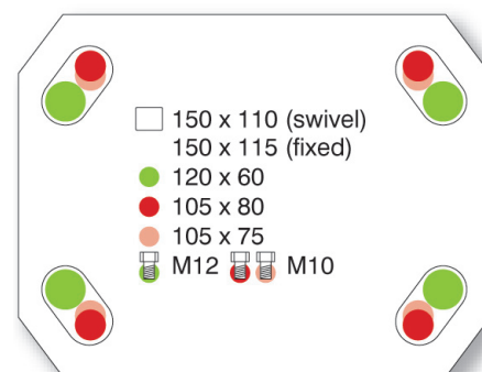
Castor top plate & hole centres
